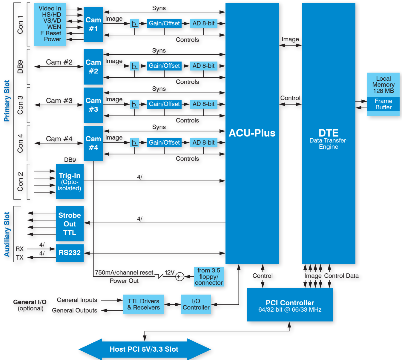
X64-AN Quad—Functional Block Diagram
