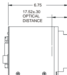
C-Mount Configuration
